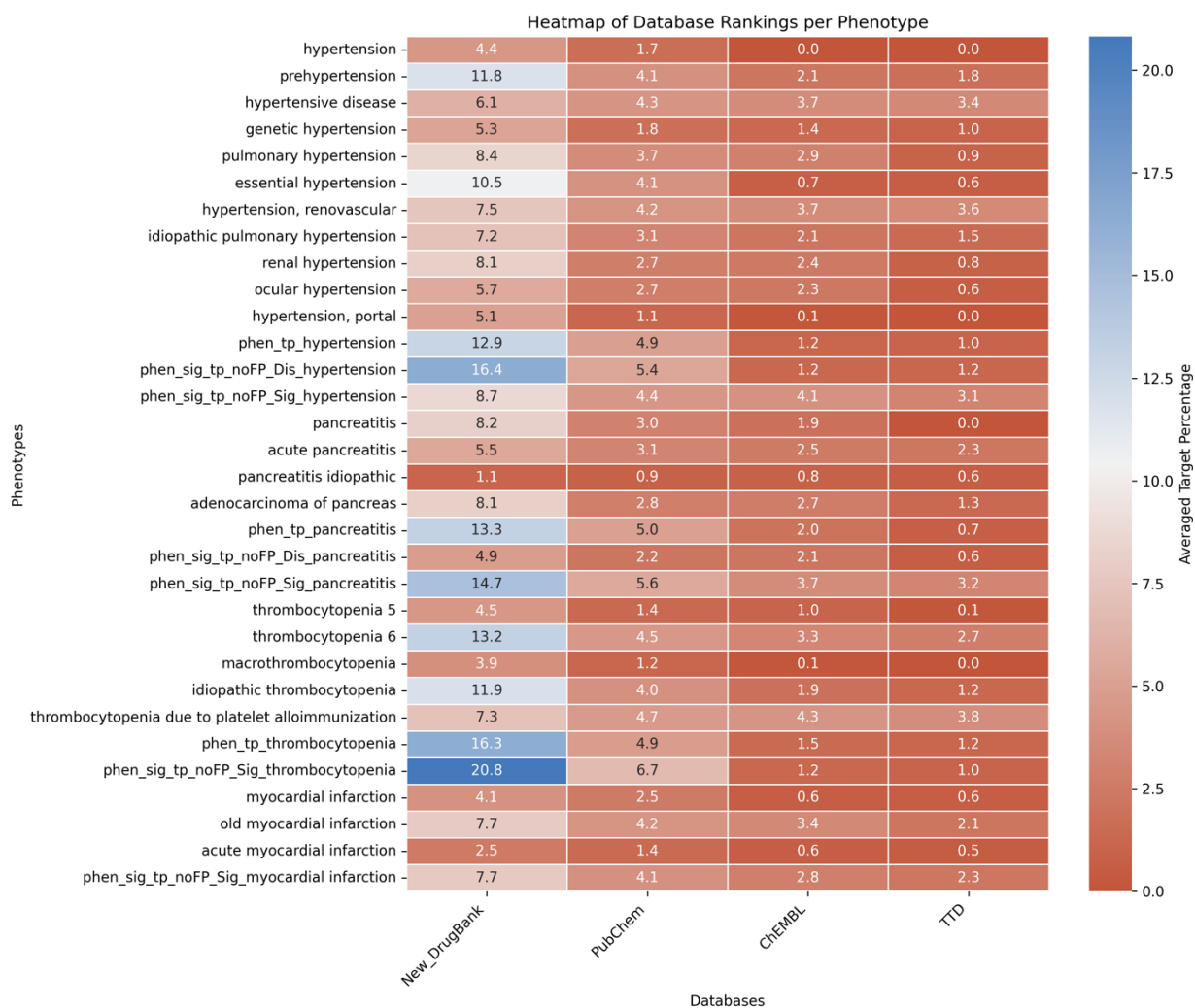
Figure S11. Heatmaps illustrating database rankings for phenotype prediction based on averaged target percentages in two filtered datasets. (a) Rankings for 111 drugs shared across TTD, New_DrugBank, ChEMBL, and STITCH (excluding PubChem and Pocket_Features). (b) Rankings for 147 drugs shared across TTD, PubChem, New_DrugBank, and ChEMBL (excluding STITCH and Pocket_Features). Blue shades indicate higher contributions of targets to phenotype prediction, while red shades signify lower contributions.
