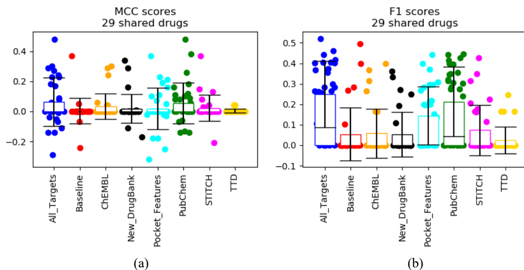
Figure S9. Additional performance metrics for 29 drugs shared across all DTI sources. We plotted Matthews Correlation Coefficients (MCC) (a), and F1 Scores (b) for 29 shared drugs for the union of all targets (blue), the baseline analysis (red), ChEMBL (orange), new DrugBank (black), PocketFEATURE (cyan), PubChem (green), STITCH (magenta), and TTD (gold). Bar charts represent the mean and standard deviation and each of the 29 drugs is represented with a single scatter point.
