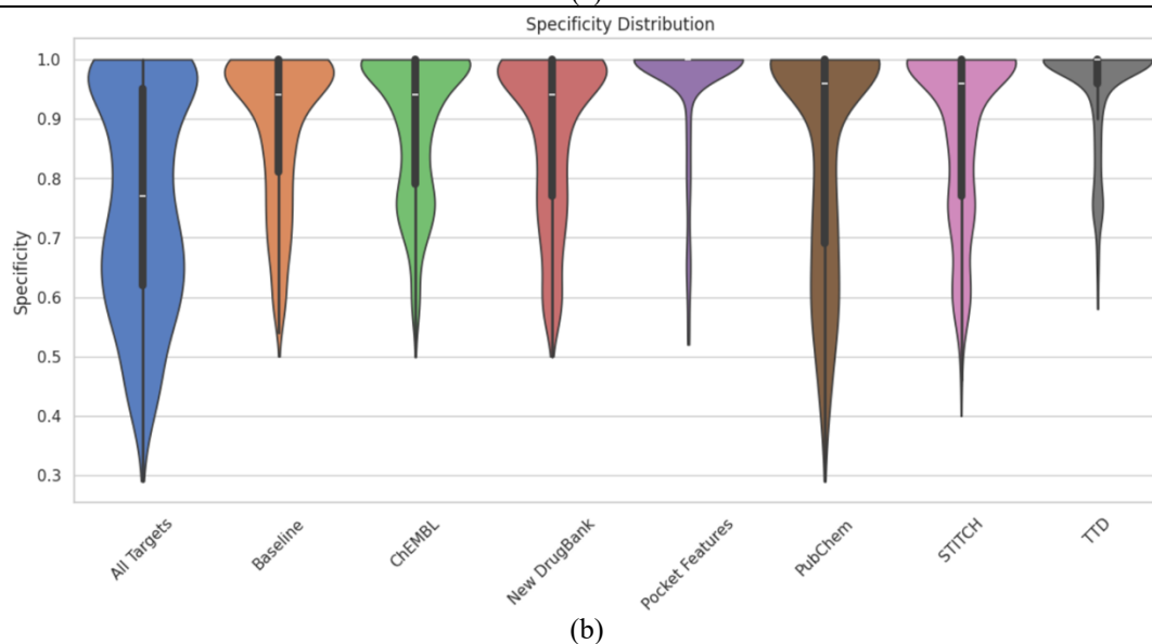
Figure S8. Violin plots illustrating the distributions of (a) sensitivity and (b) specificity for 565 drugs present in at least four databases. Sensitivity improves when combining targets from all databases, as reflected in the wider range of high-sensitivity values. Specificity remains high for individual databases but decreases when integrating all targets, demonstrating the trade-off between these metrics.
